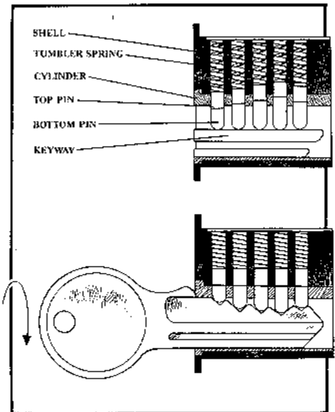
Figure 1. The pin tumbler lock, cutaway view.
