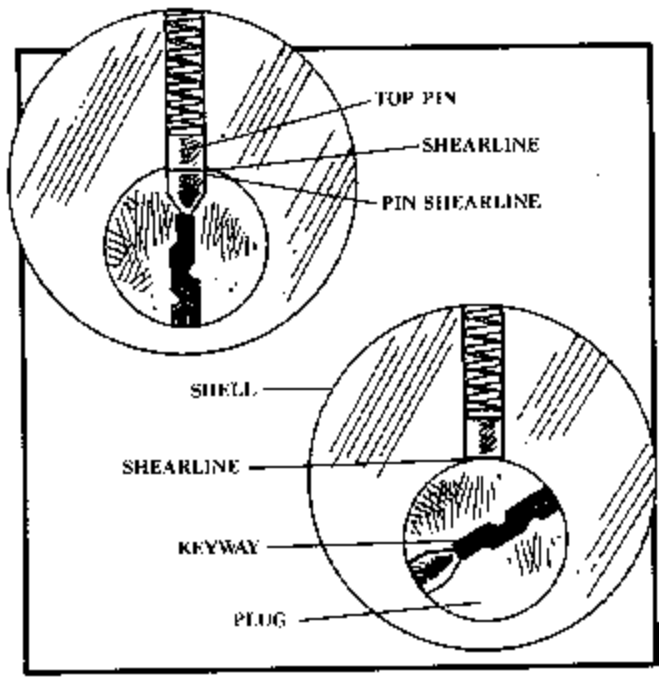
Figure 2. The pin tumbler lock, front view.
