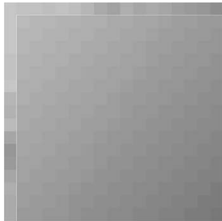
3 (plane), SAE = 2539
