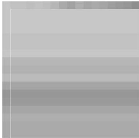
1 (horizontal), SAE = 5097
