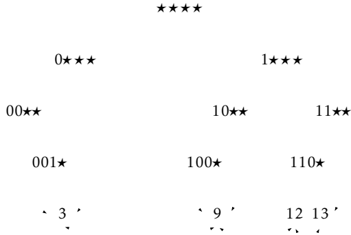
Figure 13.2: A BinaryTrie with jump pointers shown as curved dashed edges.
