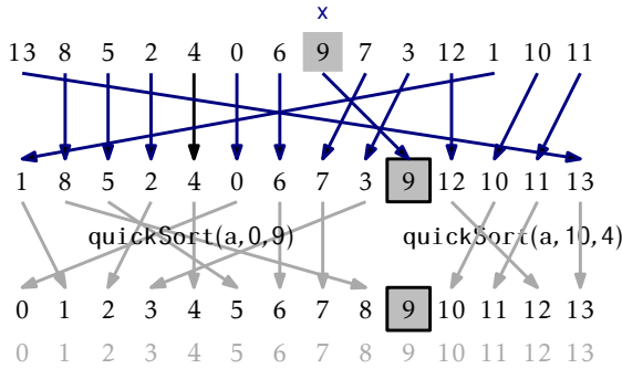
Figure 11.3: An example execution of \text{quickSort}(a, 0, 14, c)
