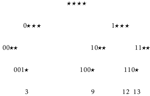
Figure 13.1: The integers stored in a binary trie are encoded as root-to-leaf paths.
