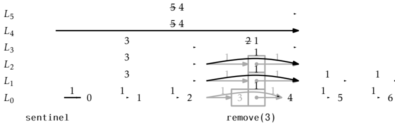
Figure 4.8: Removing an element from a SkiplistList.
