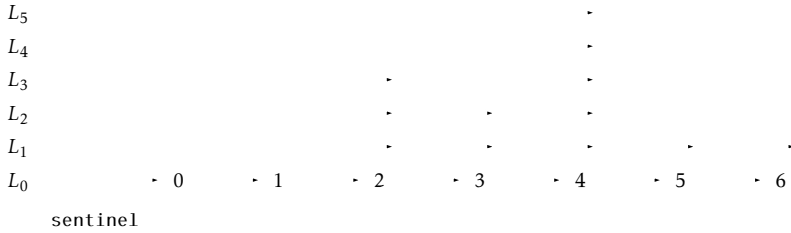
Figure 4.1: A skiplist containing seven elements.
