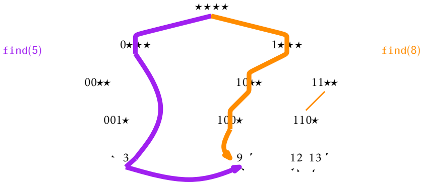
Figure 13.3: The paths followed by find(5) and find(8) .
