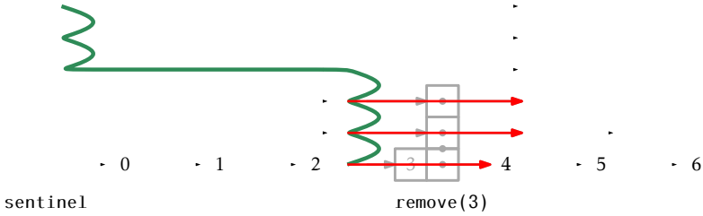
Figure 4.4: Removing the node containing 3 from a skiplist.
