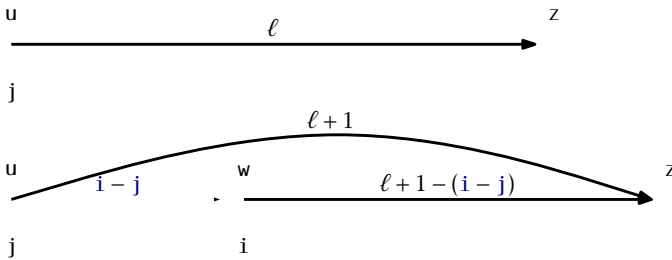
Figure 4.6: Adding an element to a SkiplistList.
