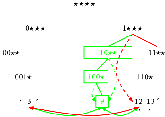
Figure 13.5: Removing the value 9 from the BinaryTrie in Figure 13.2.
