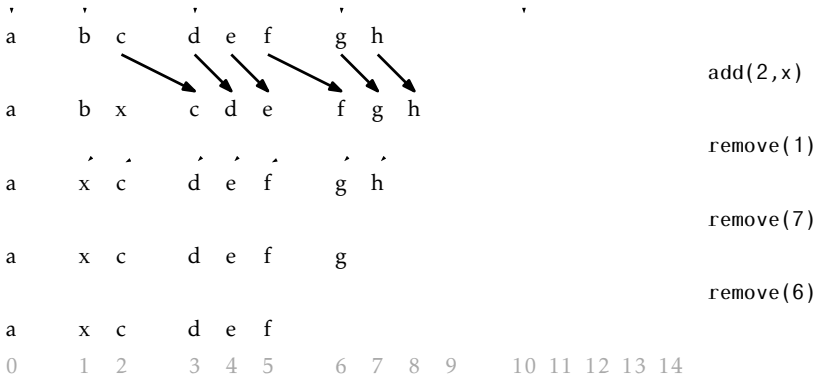
Figure 2.5: A sequence of add(i, x) and remove(i) operations on a RootishArrayStack . Arrows denote elements being copied.
