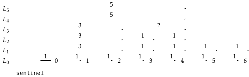
Figure 4.5: The lengths of the edges in a skiplist.
