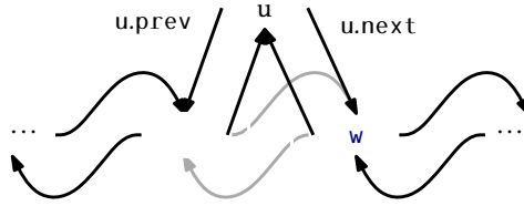
Figure 3.3: Adding the node u before the node w in a DLList.
