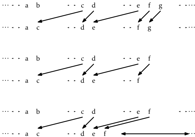
Figure 3.5: The three cases that occur during the removal of an item x in the interior of an SEList. (This SEList has block size b = 3 .)
