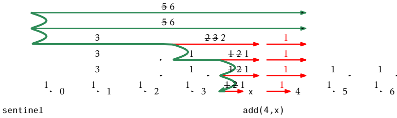
Figure 4.6: Adding an element to a SkiplistList.
