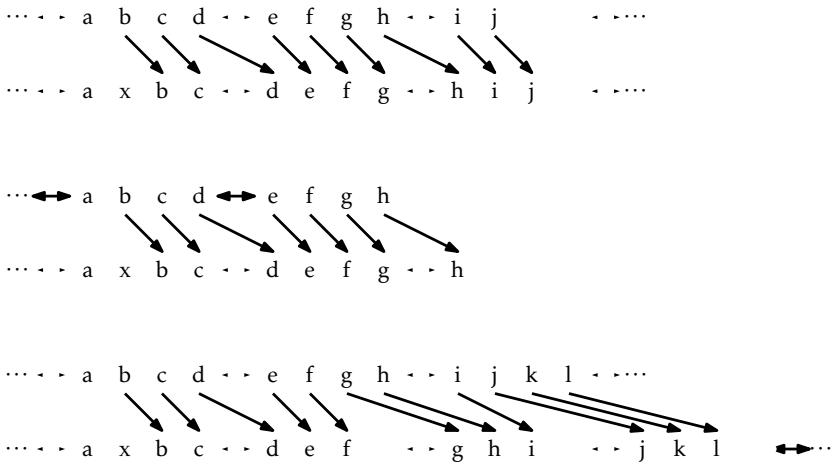
Figure 3.4: The three cases that occur during the addition of an item x in the interior of an SEList. (This SEList has block size b = 3 .)
