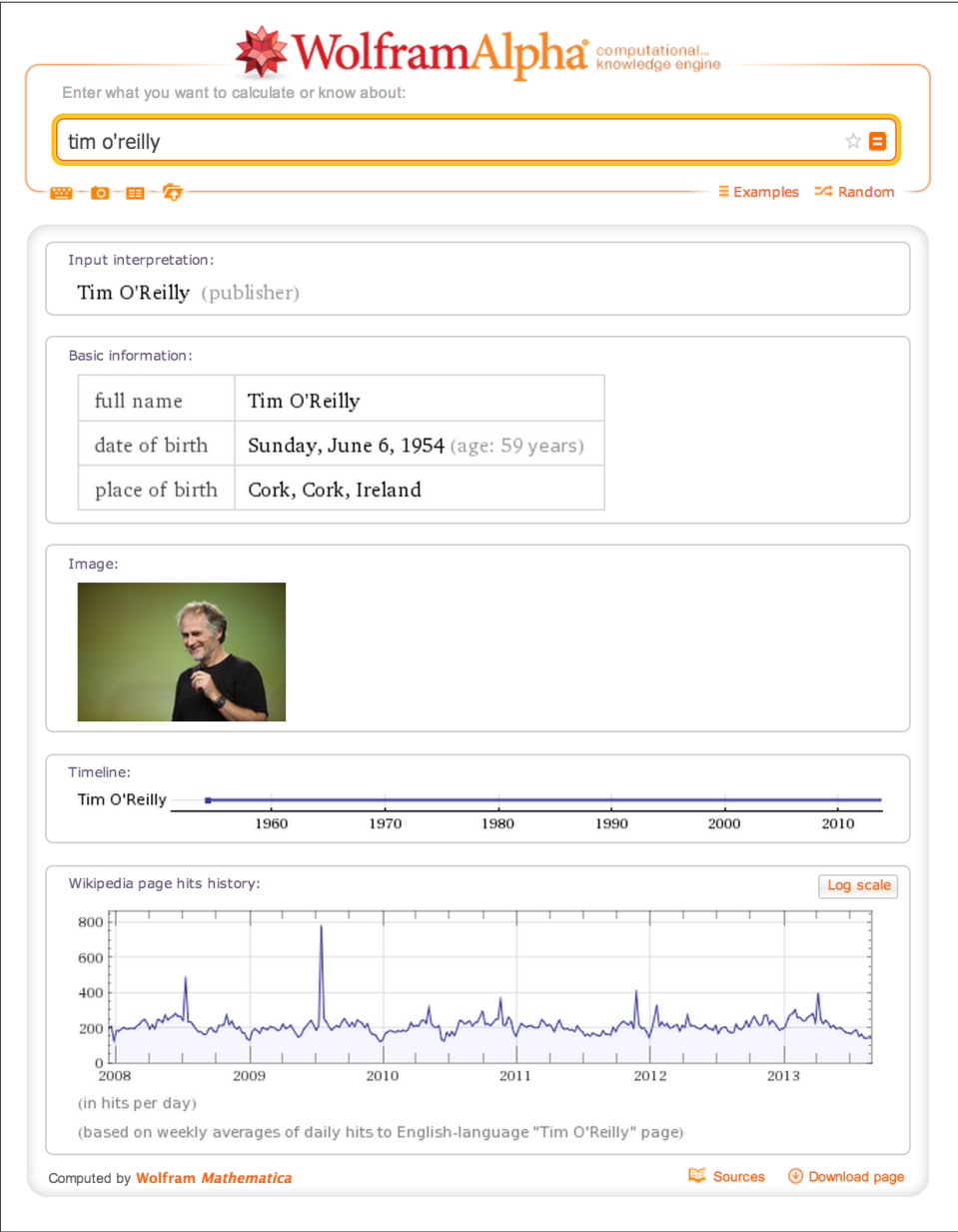
Figure 5-5. Sample results for a “tim o’reilly” query with WolframAlpha
