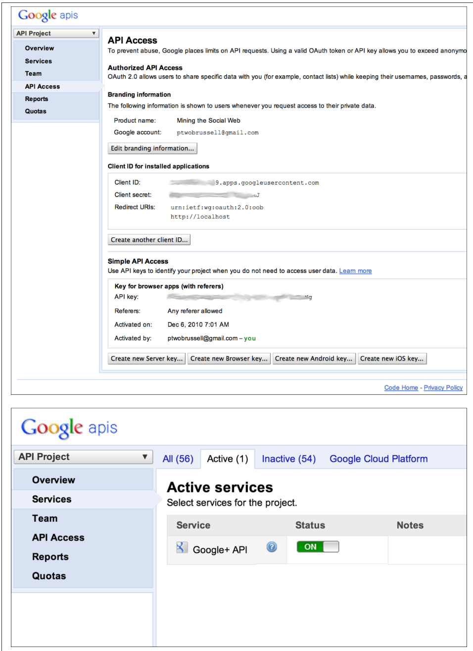
Figure 4-1. Registering an application with the Google API Console to gain API access to Google services; don't forget to enable Google+ API access as one of the service options
