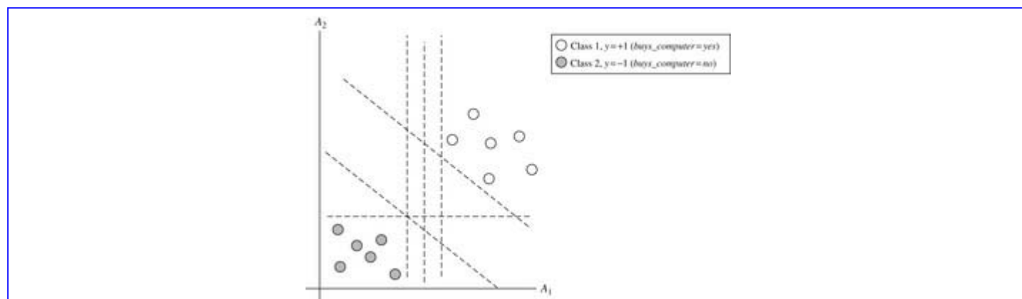
Figure 9.7 The 2-D training data are linearly separable. There are an infinite number of possible separating hyperplanes or “decision boundaries,” some of which are shown here as dashed lines. Which one is best?
