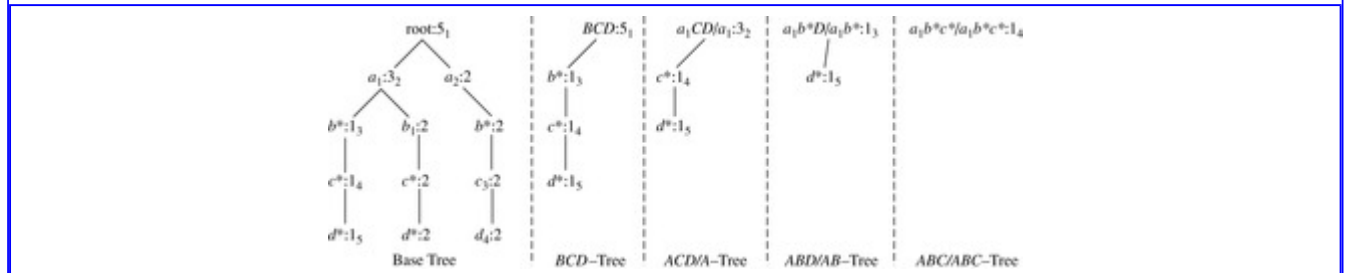
Figure 5.11 Aggregation stage one: processing the leftmost branch of the base tree.
