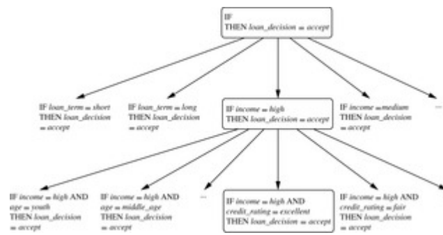
Figure 8.11 A general-to-specific search through rule space.
