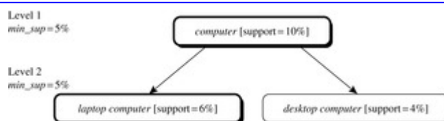
Figure 7.3 Multilevel mining with uniform support.
