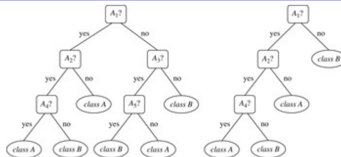
Figure 8.6 An unpruned decision tree and a pruned version of it.
