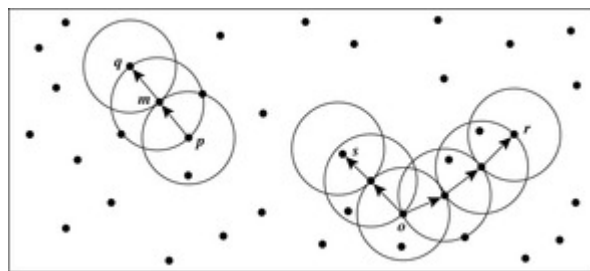
Figure 10.14 Density-reachability and density-connectivity in density-based clustering.
