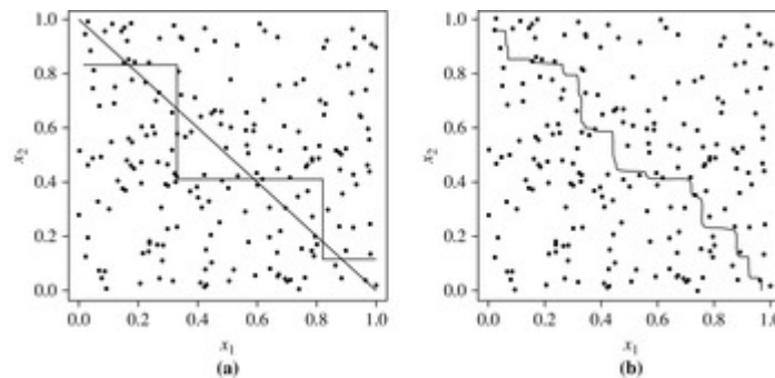
Figure 8.22 Decision boundary by (a) a single decision tree and (b) an ensemble of decision trees for a linearly separable problem (i.e., where the actual decision boundary is a straight line). The decision tree struggles with approximating a linear boundary. The decision boundary of the ensemble is closer to the true boundary.
