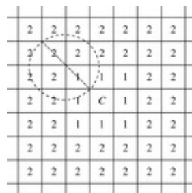
Figure 12.7 Grids in the CELL method.
