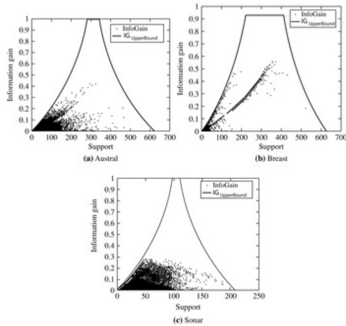
Figure 9.12 Information gain versus pattern frequency (support) for three UCI data sets. A theoretical upper bound on information gain ( IG_{Upper\ Bound} ) is also shown. Source: Adapted from Cheng, Yan, Han, and Hsu [CYHH07].
