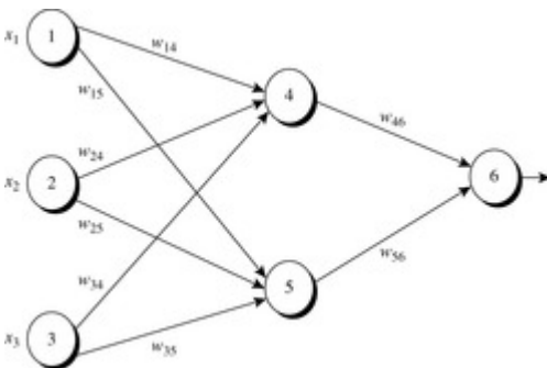
Figure 9.5 Example of a multilayer feed-forward neural network.
