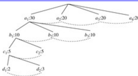
Figure 5.9 Base cuboid tree fragment.
