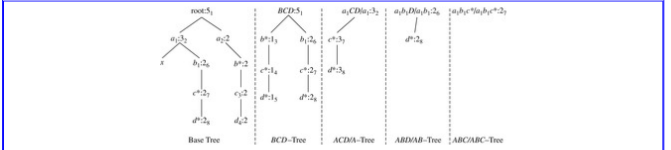
Figure 5.12 Aggregation stage two: processing the second branch of the base tree.
