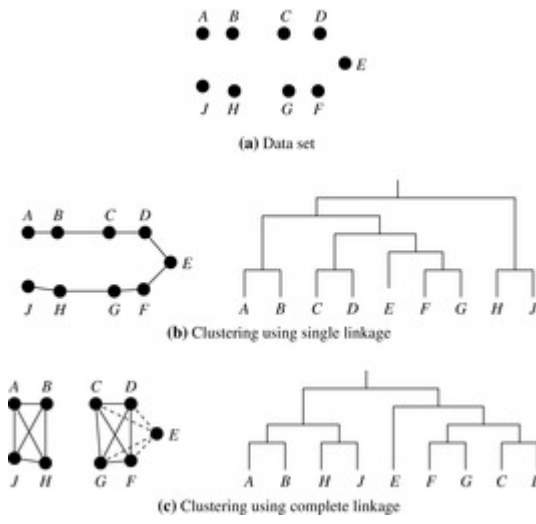
Figure 10.8 Hierarchical clustering using single and complete linkages.
