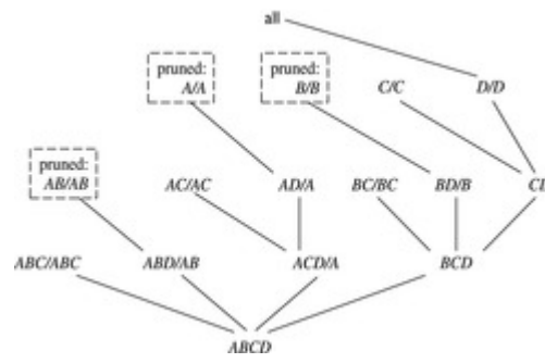
Figure 5.8 Star-Cubing: bottom-up computation with top-down expansion of shared dimensions.
