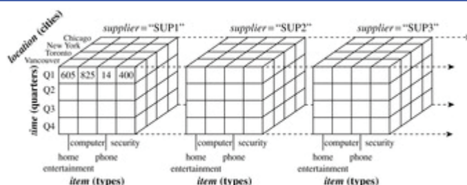
Figure 4.4 A 4-D data cube representation of sales data, according to time , item , location , and supplier . The measure displayed is dollars_sold (in thousands). For improved readability, only some of the cube values are shown.
