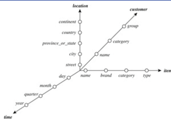
Figure 4.13 A starnet model of business queries.
