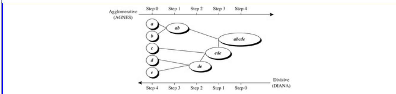
Figure 10.6 Agglomerative and divisive hierarchical clustering on data objects \{a, b, c, d, e\} .
