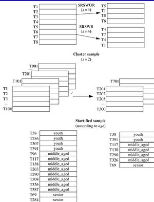
Figure 3.9 Sampling can be used for data reduction.
