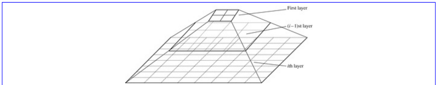
Figure 10.19 Hierarchical structure for STING clustering.
