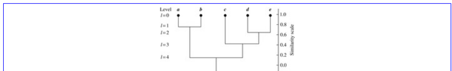
Figure 10.7 Dendrogram representation for hierarchical clustering of data objects \{a, b, c, d, e\} .
