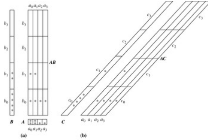
Figure 5.4 Memory allocation and computation order for computing Example 5.4 's 1-D cuboids. (a) The 1-D cuboids, A and B , are aggregated during the computation of the smallest 2-D cuboid, AB . (b) The 1-D cuboid, C , is aggregated during the computation of the second smallest 2-D cuboid, AC . The *'s represent chunks that, so far, have been aggregated to.
