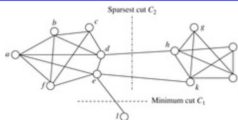
Figure 11.14 A graph G and two cuts.
