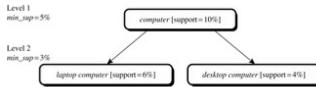
Figure 7.4 Multilevel mining with reduced support.
