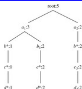
Figure 5.10 Compressed base table star-tree.
