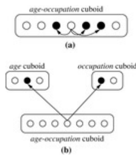
Figure 5.15 Query expansion within sampling cube: Given small data samples, both methods use strategies to boost the reliability of query answers by considering additional data cell values. (a) Intracuboid expansion considers nearby cells in the same cuboid as the queried cell. (b) Intercuboid expansion considers more general cells from parent cuboids.
