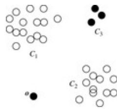
Figure 12.12 Outliers in small clusters.
