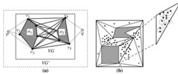
Figure 11.16 Clustering with obstacle objects ( o_1 and o_2 ): (a) a visibility graph and (b) triangulation of regions with microclusters.
