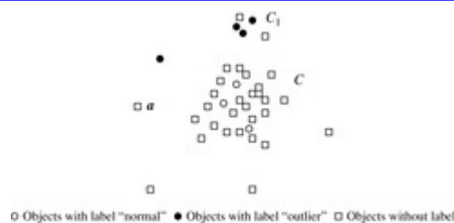
Figure 12.14 Detecting outliers by semi-supervised learning.
