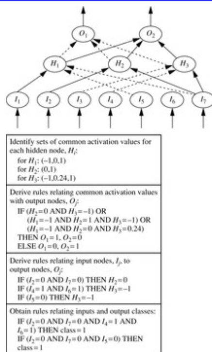
Figure 9.6 Rules can be extracted from training neural networks.
