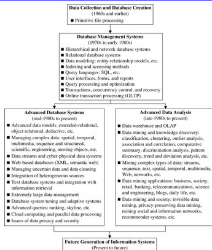
Figure 1.1 The evolution of database system technology.
