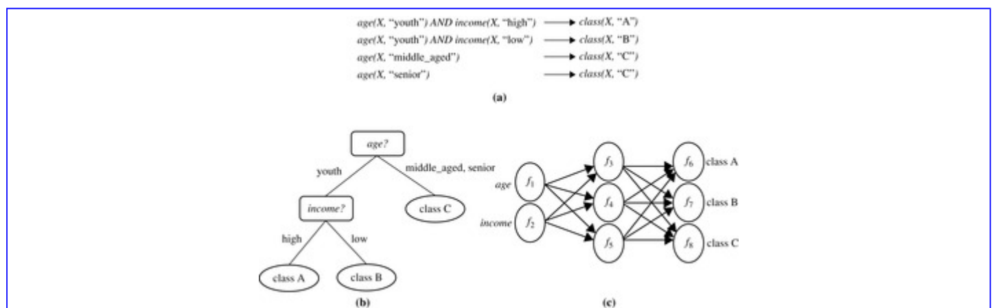
Figure 1.9 A classification model can be represented in various forms: (a) IF-THEN rules, (b) a decision tree, or (c) a neural network.
