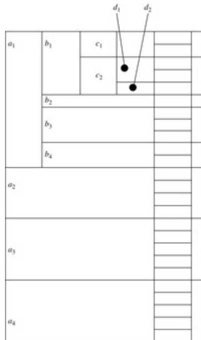
Figure 5.7 BUC partitioning snapshot given an example 4-D data set.
