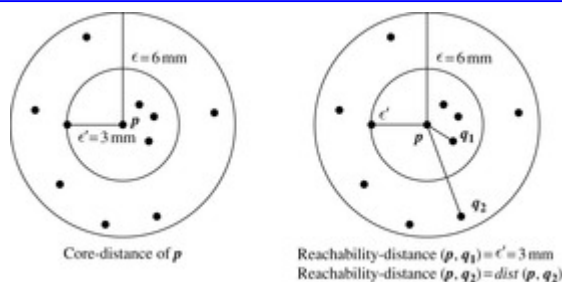
Figure 10.16 OPTICS terminology.
