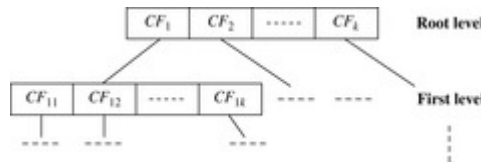
Figure 10.9 CF-tree structure.
