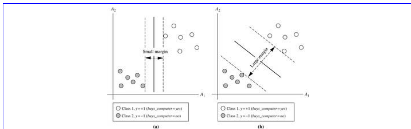
Figure 9.8 Here we see just two possible separating hyperplanes and their associated margins. Which one is better? The one with the larger margin (b) should have greater generalization accuracy.
