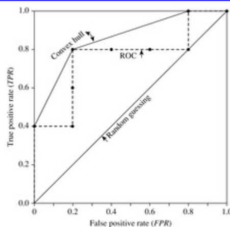
Figure 8.19 ROC curve for the data in Figure 8.18.
