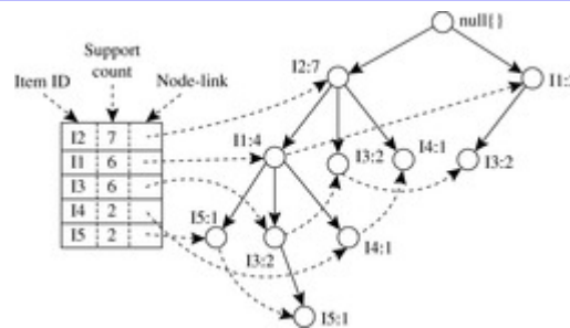
Figure 6.7 An FP-tree registers compressed, frequent pattern information.
