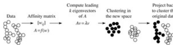
Figure 11.10 The framework of spectral clustering approaches.
