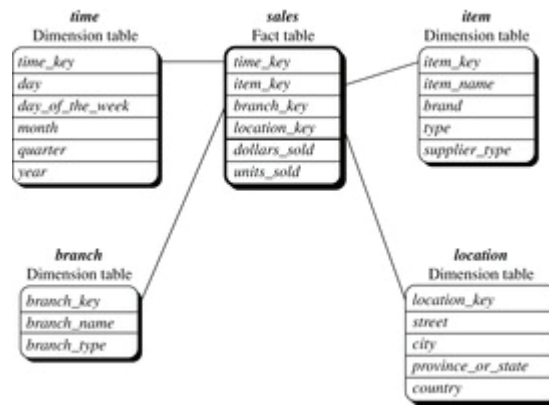
Figure 4.6 Star schema of sales data warehouse.
