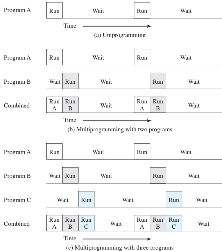
Figure 2.5 Multiprogramming Example
