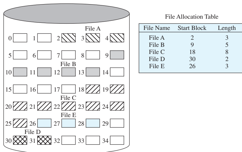
Figure 12.7 Contiguous File Allocation
